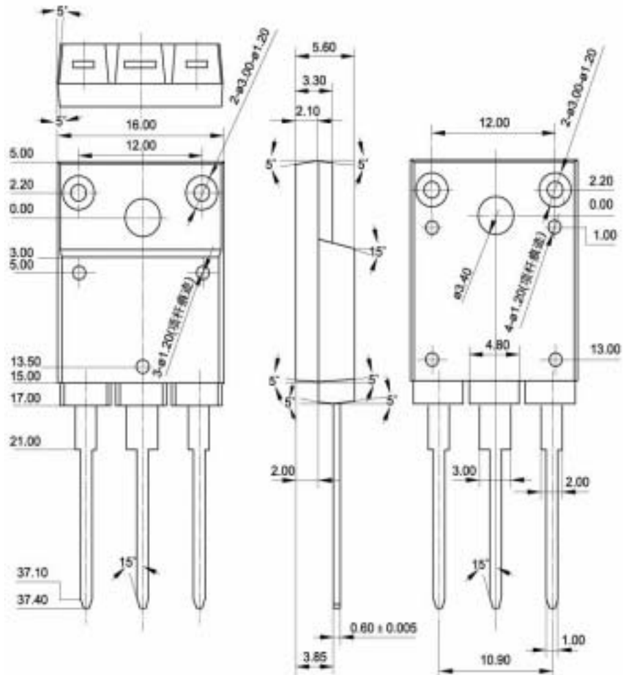
Fig.2 Outline dimensions
